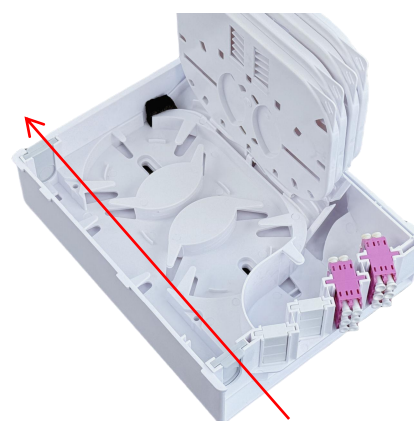
1 / 1 In-line Ports × Ø15mm
