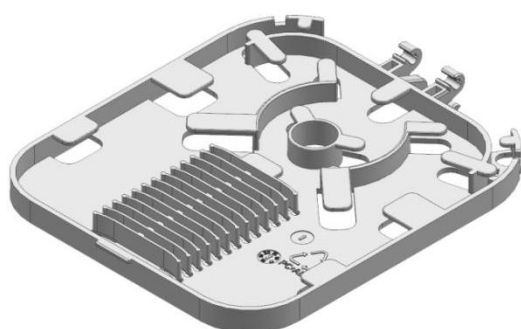
12 Fibers/Tray Suitable for 1×8 Micro PLC Splitter
